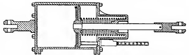
THE SCHROYER-THOMPSON PISTON-TRAVEL INDICATOR.
